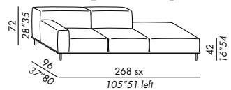
terminale penisola - peninsula end unit 270
